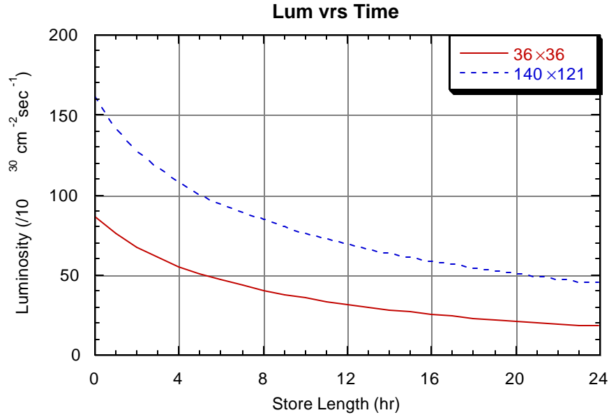
Figure 1.3. Predicted time evolution of luminosity for the two sets of store parameters listed in Table 1.1.
