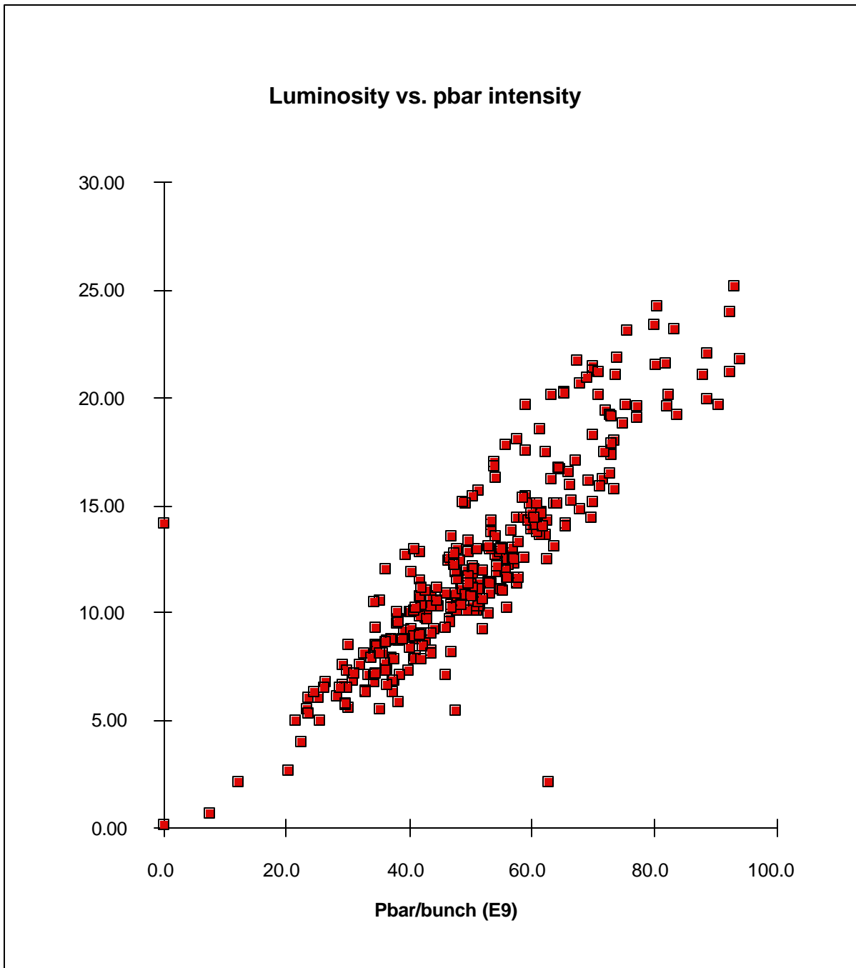
Figure 1.1. Luminosity observed in Run Ib vs. antiproton bunch intensity for all stores over the period July 23, 1994-July 9, 1995.
