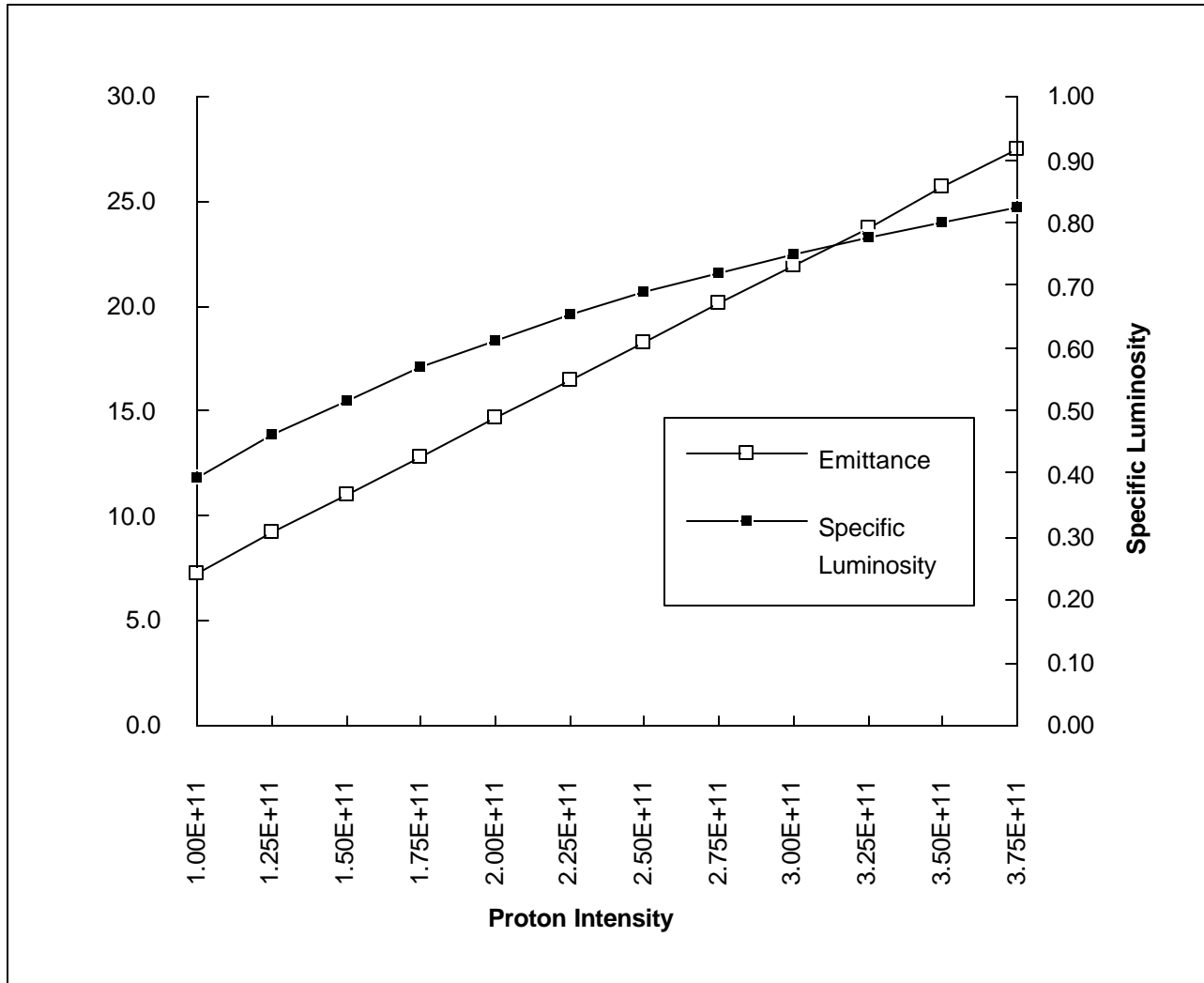
Figure 1.2. Proton emittance (mm-mrad) and luminosity per antiproton (arbitrary units) for the beam-beam limited situation. The head-on beam-beam tune shift seen by the antiprotons is .022 and the antiproton beam emittance 15\pi mm-mrad in this case. Long range beam-beam interactions are ignored.
